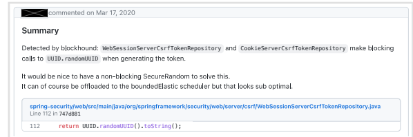
Figure 5: Blocking call due to an improper use of a Java utility [8].
