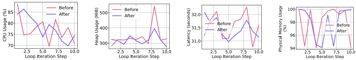
Figure 7: Performance measurement over 10 loops after fixing blocking calls in Apache James Project [16].
